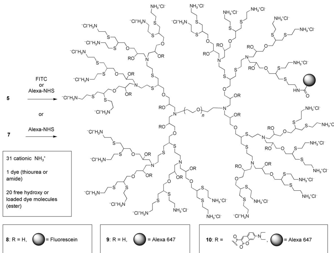
Scheme 2. Synthesis of labeled dendrimers [G-4]-FITC ( 8 ), [G-4]-Alexa ( 9 ), and [G-4]-(coumarin) 20 -Alexa ( 10 ). FITC = fluorescein isothiocyanate.
