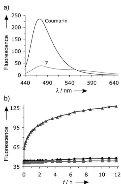
Figure 2. a) Fluorescence spectra of free coumarin and [G-4]-(coumarin) 20 ( 7 ). b) Fluorescence intensity of 7 at 480 nm as a function of time in the presence of esterase at pH 7.4 ( \blacktriangle ) and in the absence of esterase at pH 5.0 ( \blacksquare ) and 7.4 ( \blacklozenge ).
